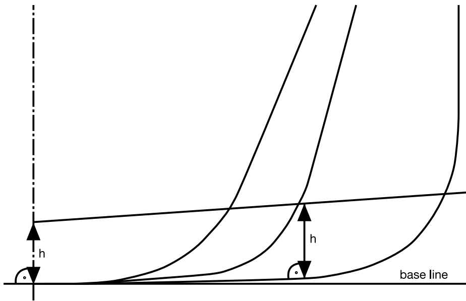
Figure 3 – Cargo tank boundary lines for the purpose of paragraph 6
