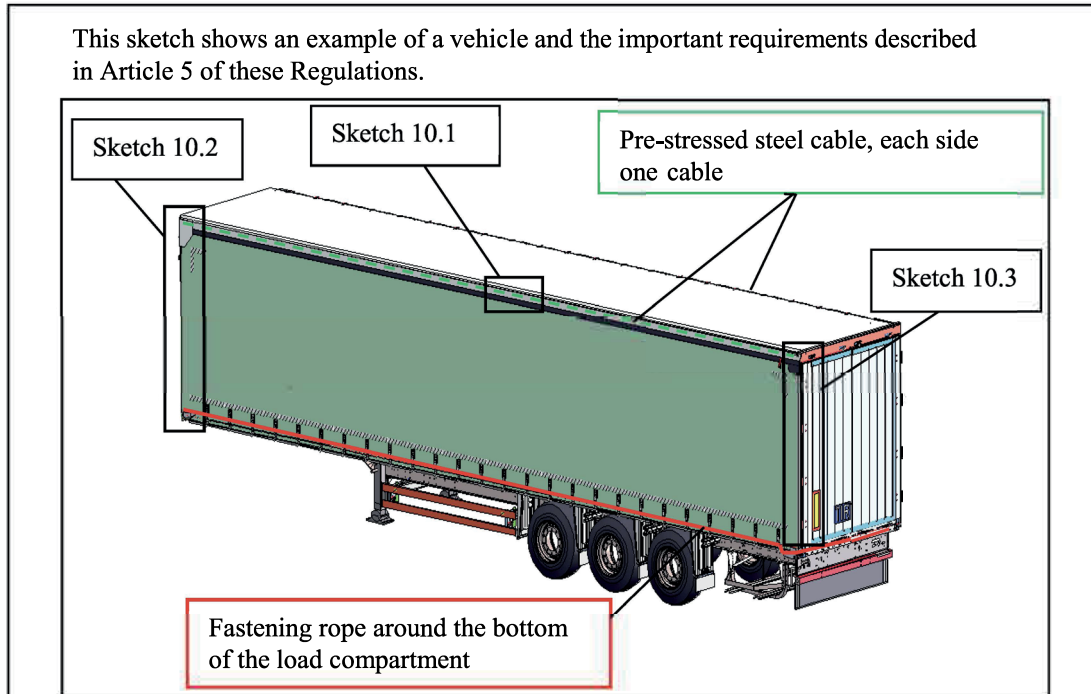
Sketch No. 10.1
